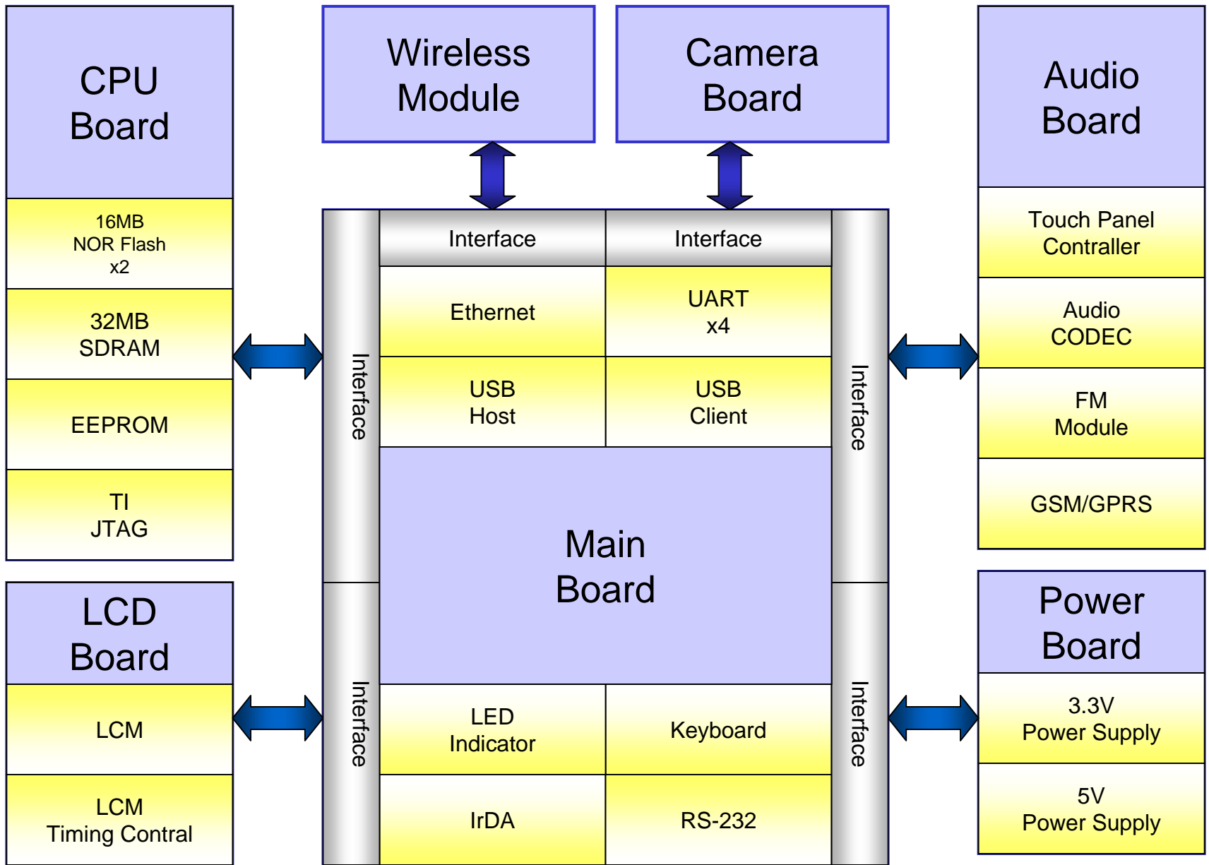
OMAP 5910 EVM BOARD FUNCTIONAL BLOCK DIAGRAM
