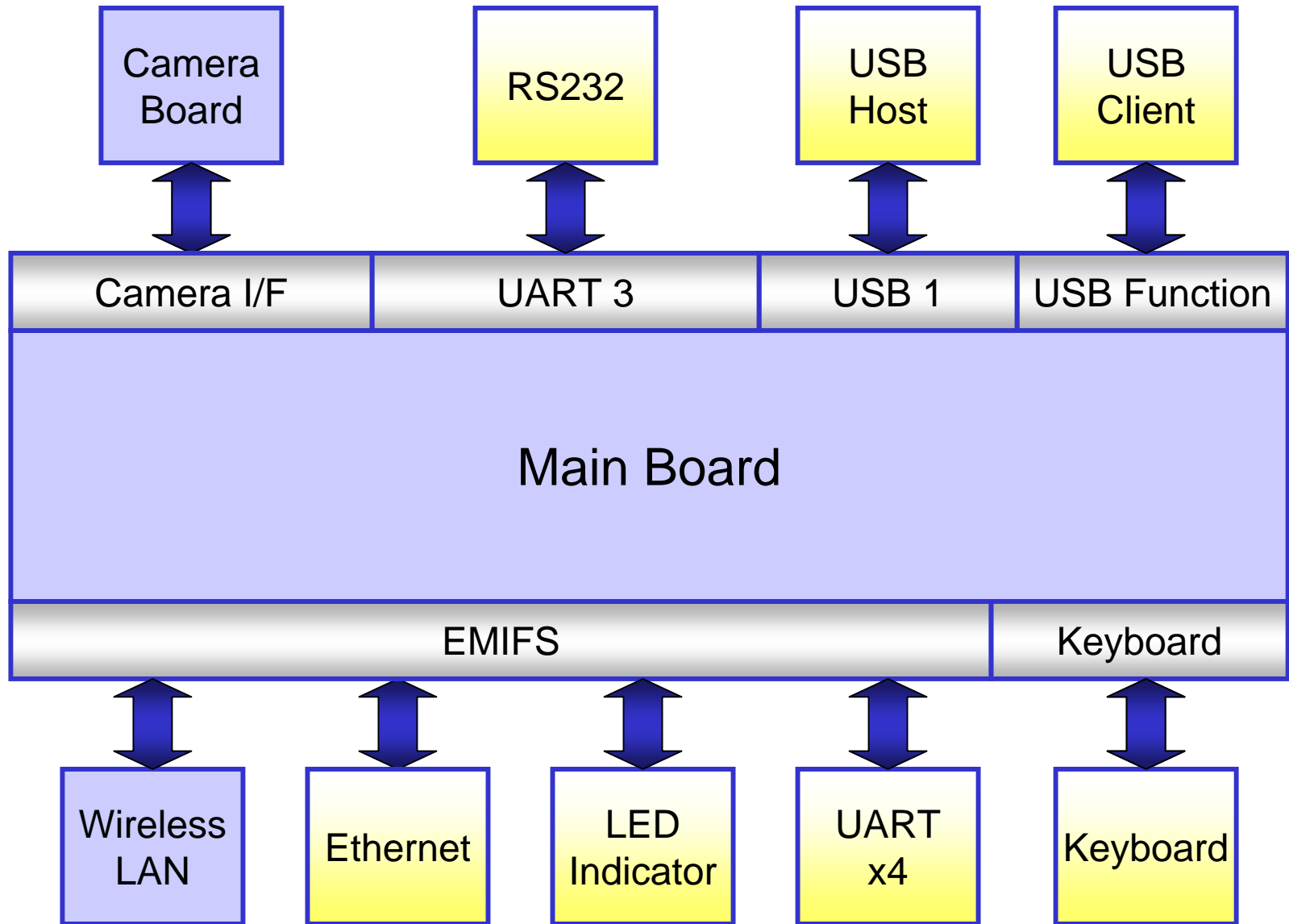
MAIN BOARD FUNCTIONAL BLOCK DIAGRAM
